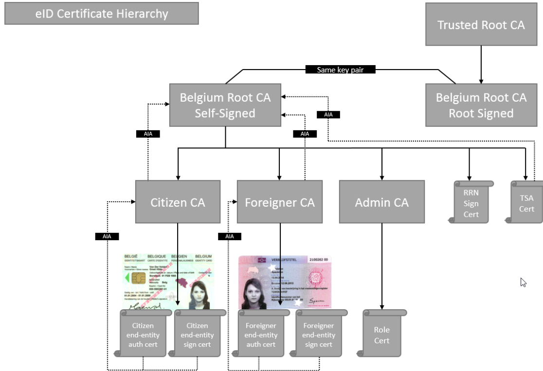
Figure: Belgian eID PKI Hierarchy
