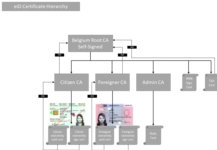
Figure: Belgian eID PKI Hierarchy
